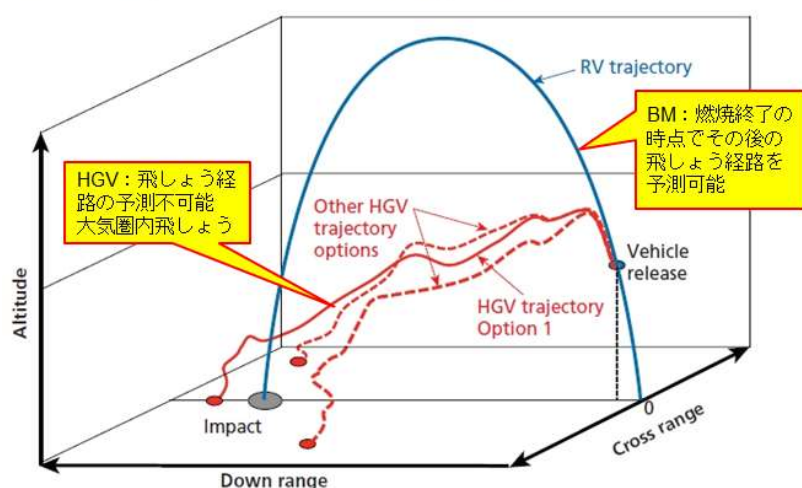
Figure 1.3 Ballistic Reentry Vehicle (RV) Versus HGV Trajectories
